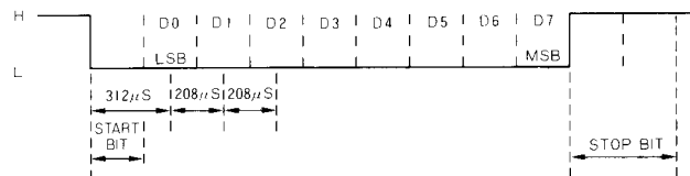
Data Format for 1 Character
