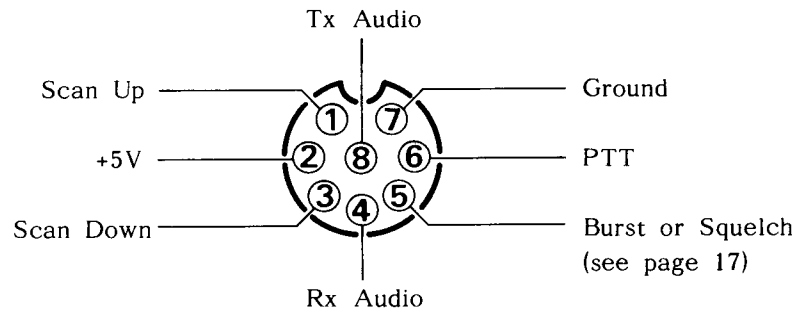
MIC Jack Pinout
