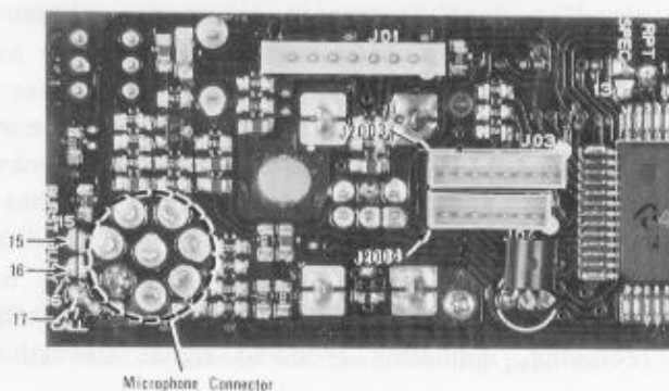
Microphone Connector
